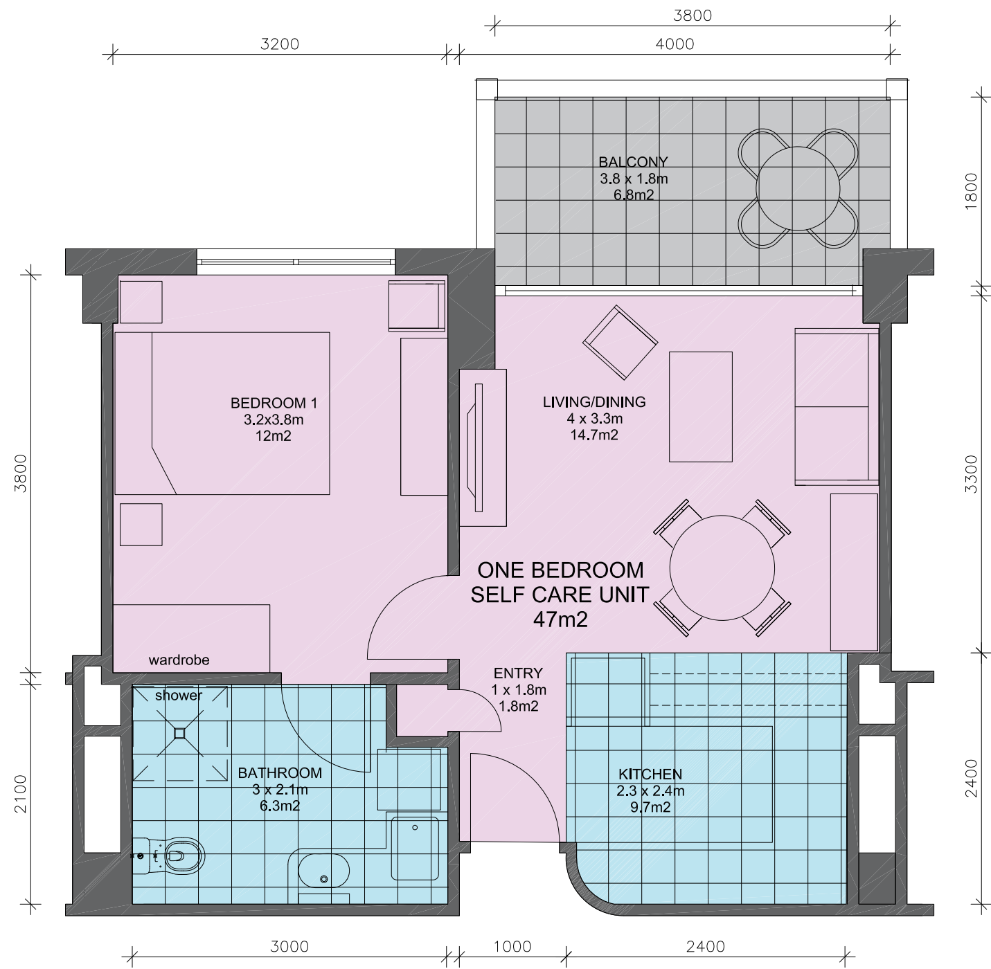
1 MARKETING PLAN – 1 BEDROOM SELF CARE UNIT 1:50
